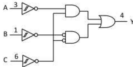
Fig. 1. Logic symbol
