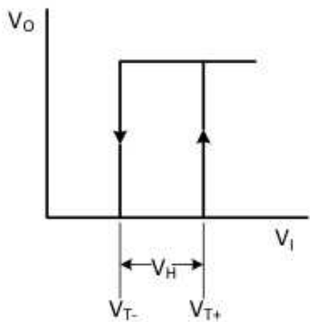
Fig. 14. Transfer characteristic
