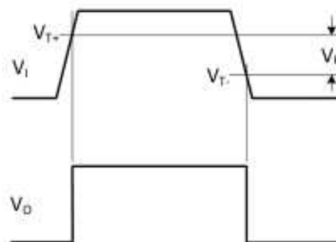
Fig. 13. Definition of V_{T+} , V_{T-} and V_H
