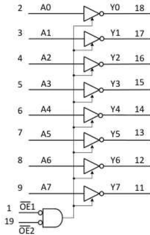
Fig. 2. Functional diagram
