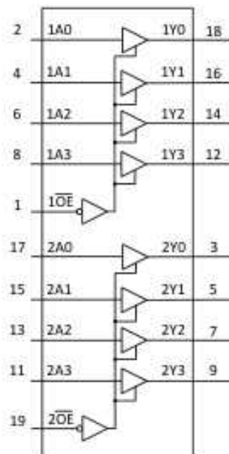
Fig. 1. Functional diagram
