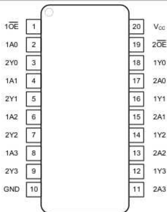
Fig. 4. Top view pin configuration SOP, SSOP and TSSOP
