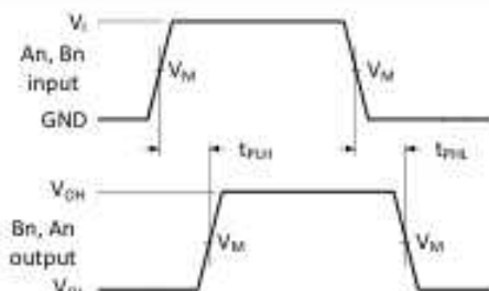
Fig. 4. Input (An, Bn) to output (Bn, An) propagation delays and output transition times
