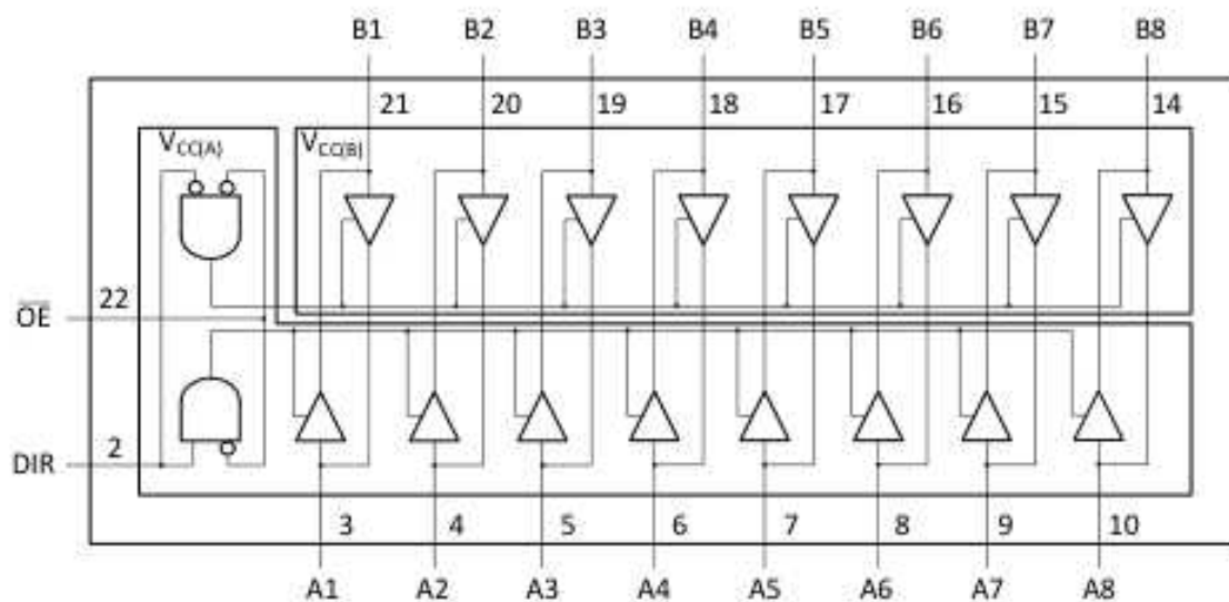
Fig. 1. Logic symbol
