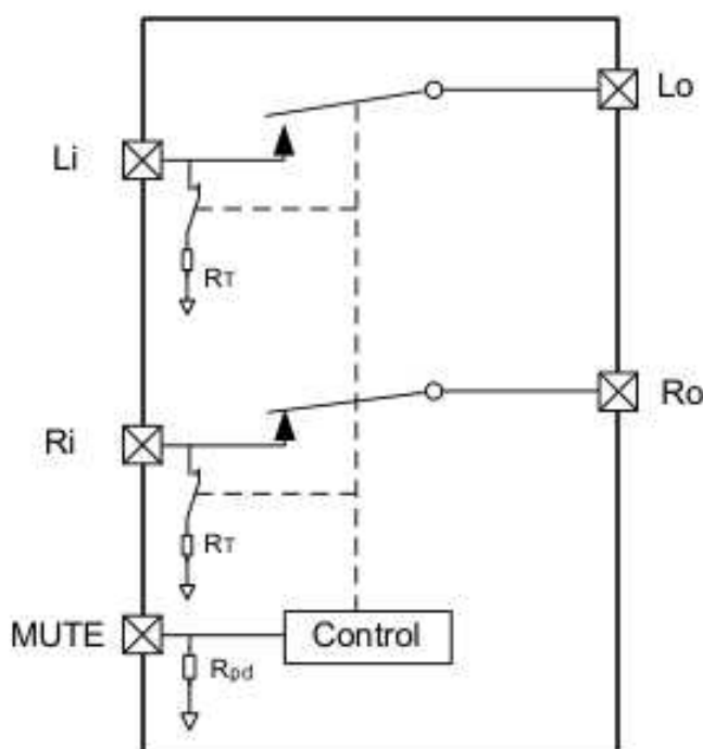
Fig 1. Function Diagram
