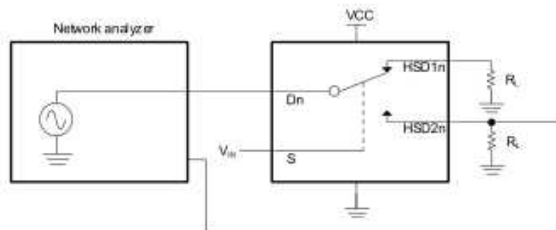
Fig 6. Off isolation
