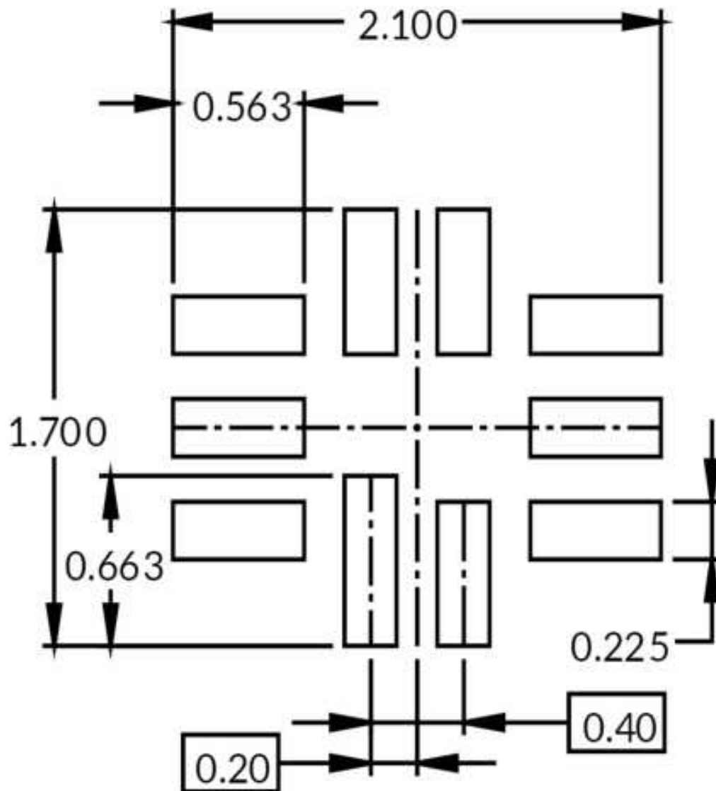
RECOMMENDED LAND PATTERN
