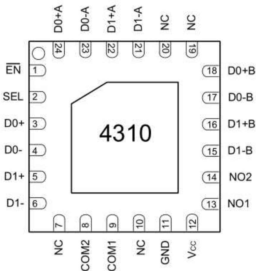
Fig. 1. Top view pin configuration QFN 4 × 4-24L
