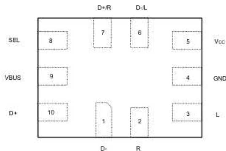
Fig. 1. Top view pin configuration QFN 1.4x1.8-10L
