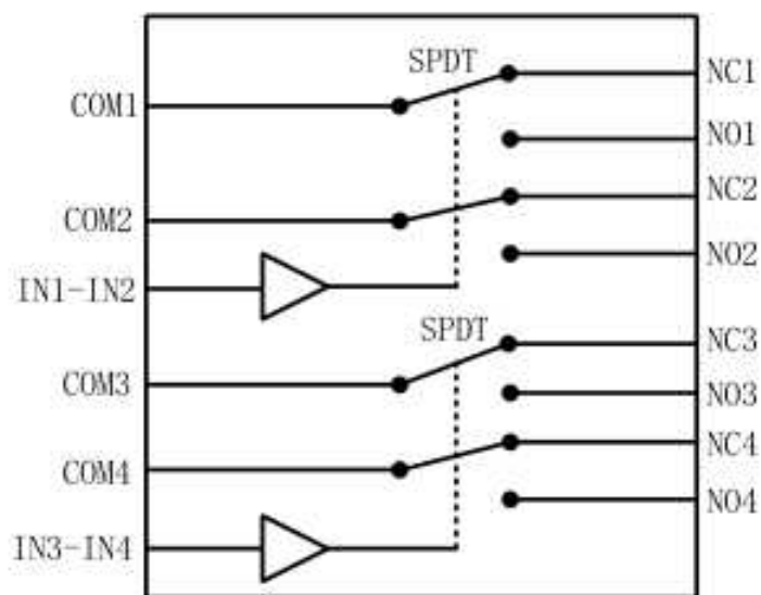
Fig. 2. Functional Block Diagram
