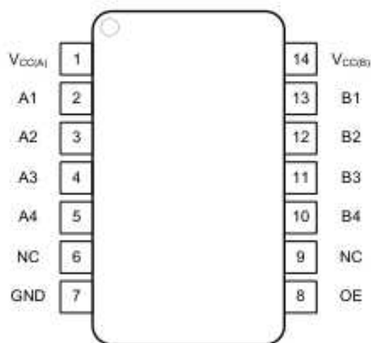
Fig. 2. Top view pin configuration TSSOP and SOP
