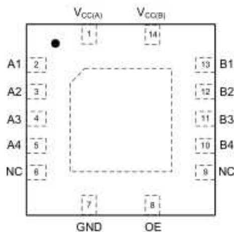
Fig. 3. Top view pin configuration QFN14L
