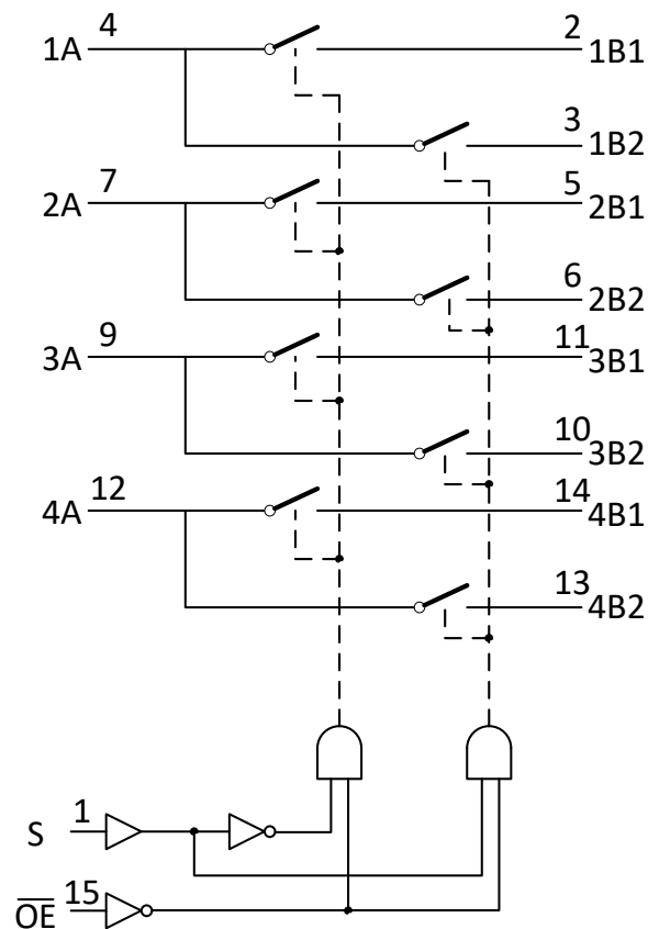
Fig. 1. Logic diagram
