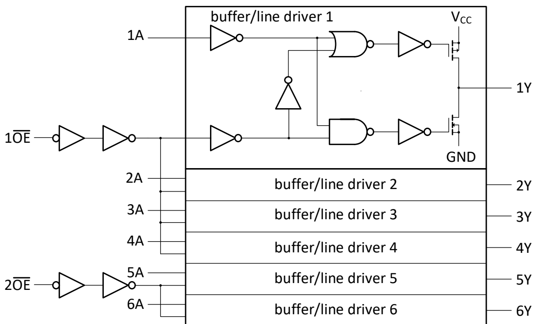
Fig. 3. Logic diagram
