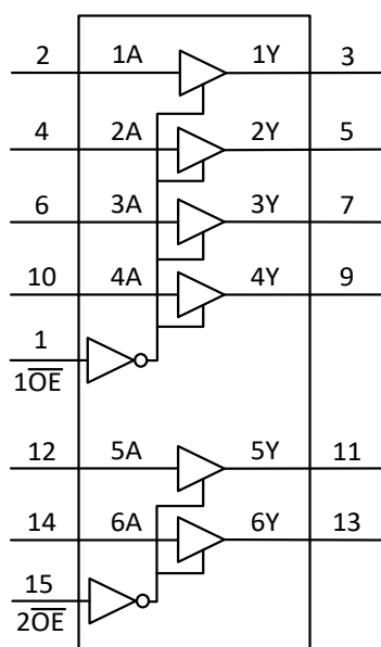
Fig. 1. Functional diagram
