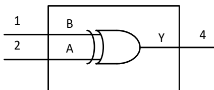
Fig. 1. Logic symbol
