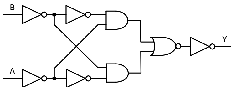
Fig. 3. Logic diagram
