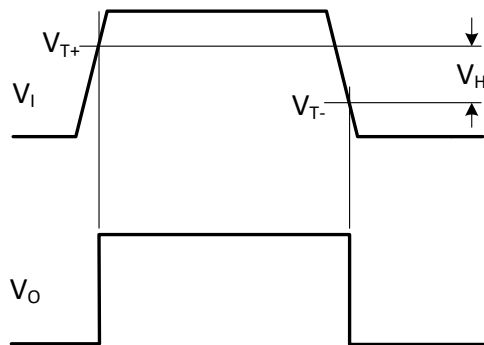
Fig. 15. Definition of V_{T+} , V_{T-} and V_H
