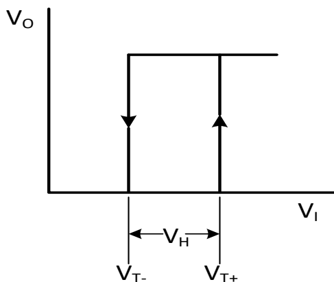
Fig. 14. Transfer characteristic
