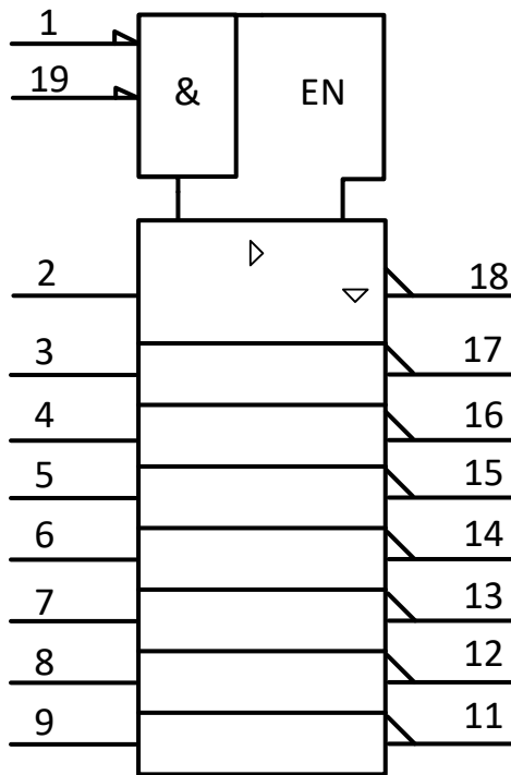
Fig. 1. IEC logic symbol
