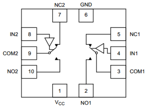
Fig 1. Top view pin configuration QFN-10L
