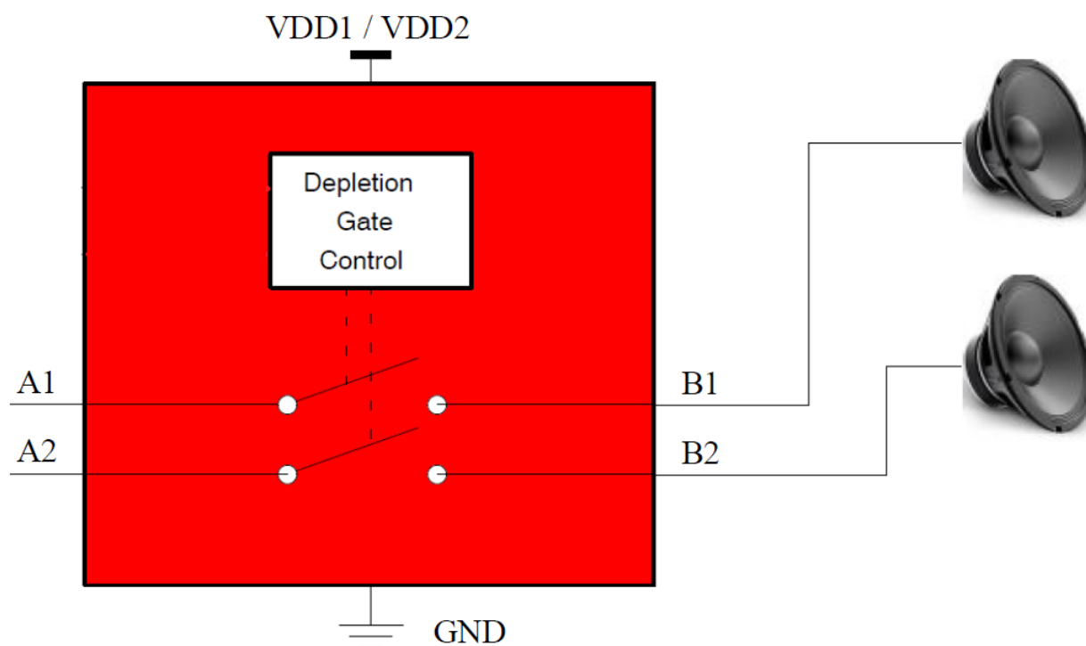
Fig 1. Function Diagram
