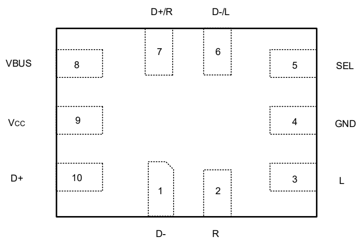
Fig. 1. Top view pin configuration QFN 1.4×1.8-10L
