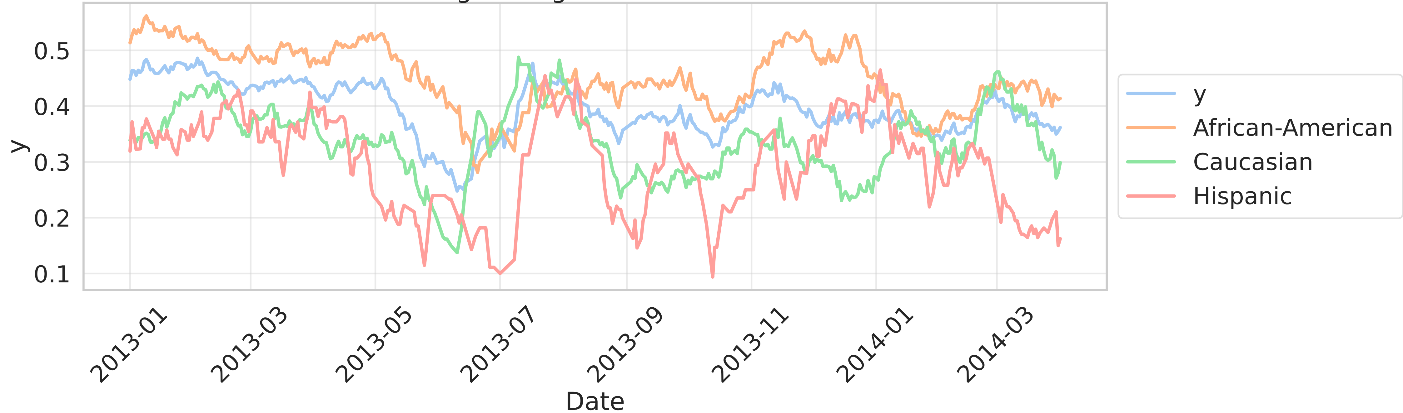
Moving average of recidivism rate
