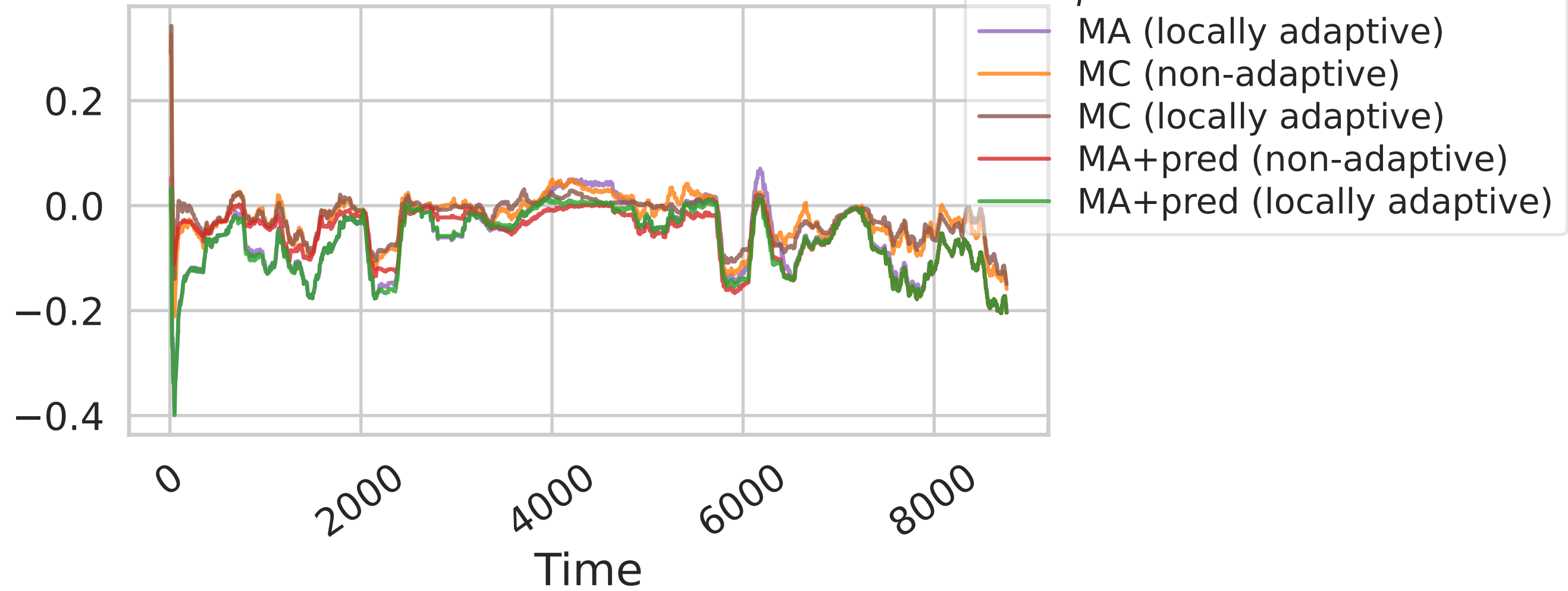
Prediction error
