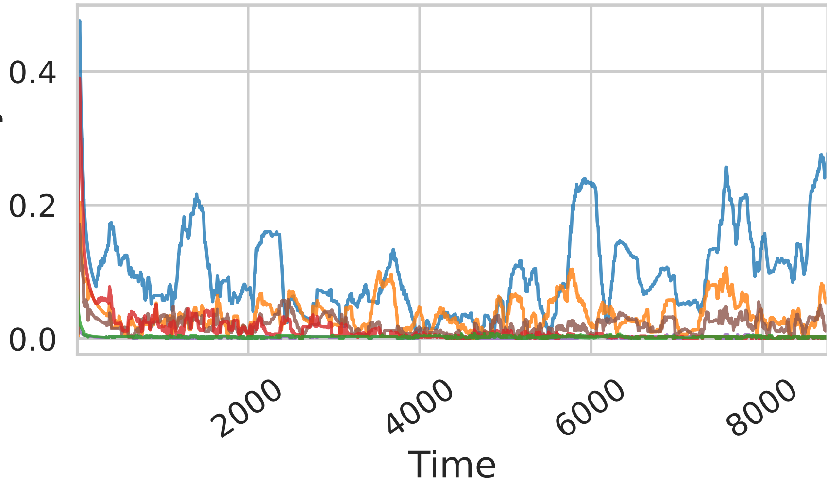
Multiaccuracy error
