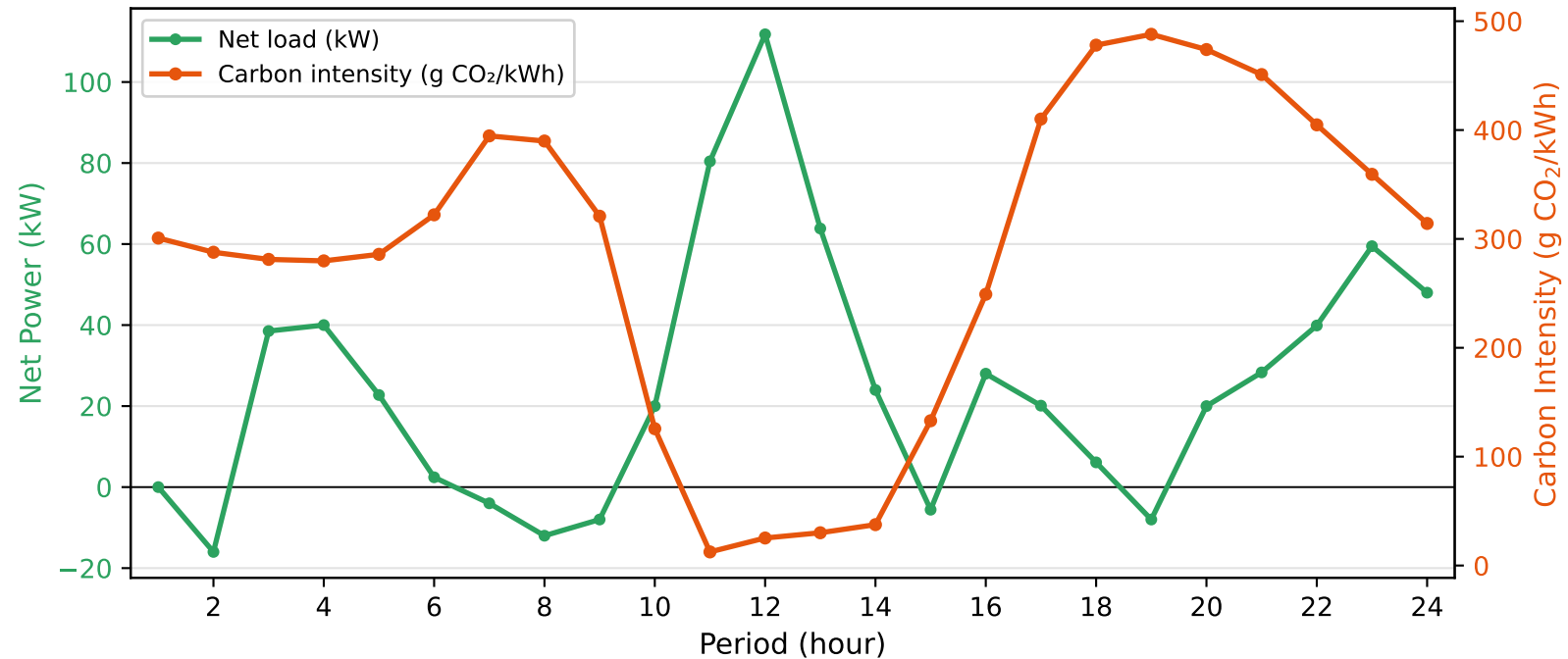
Aggregate Fleet Load vs Carbon Intensity — Carbon-Only Scheme ( \beta = 1 )
