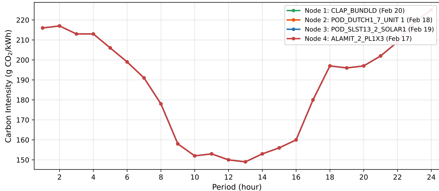
Nodal Carbon Intensity Profiles — 4 Nodes × 4 Dates (Each node assigned a distinct date profile from CAISO data)
