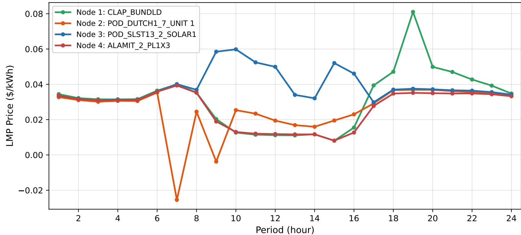
Nodal LMP Price Profiles — All 4 Charging Nodes
