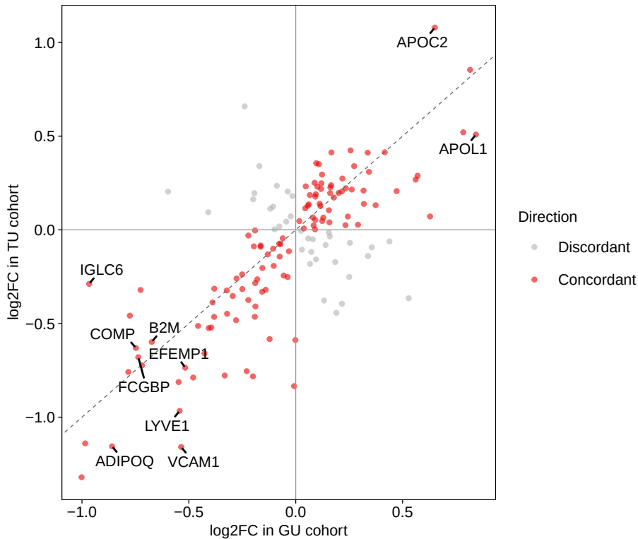
Cross-cohort log2FC concordance ( r=0.73 )
