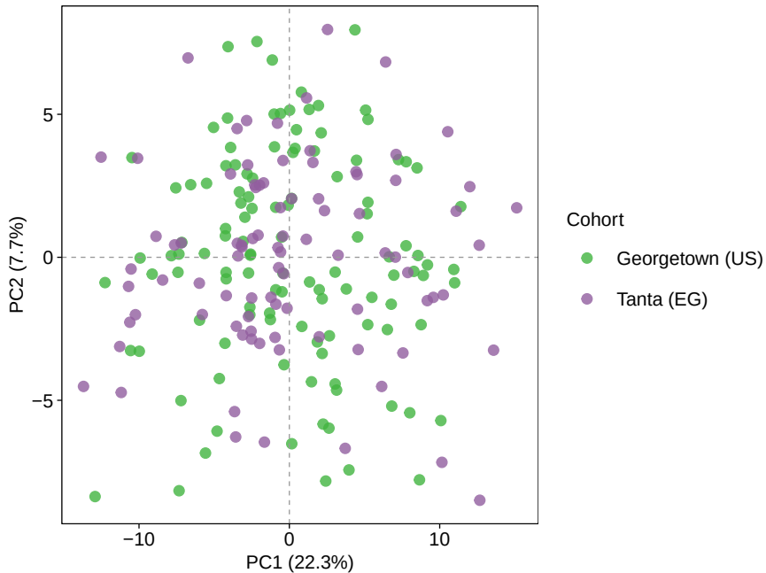
PCA scores – colour = cohort
