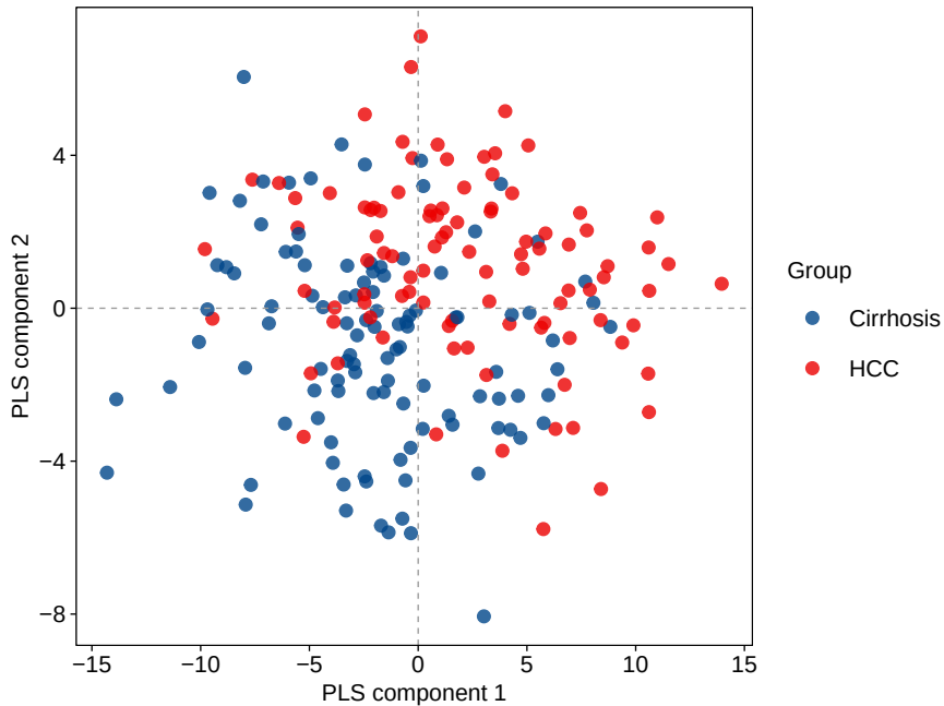
PLS-DA scores (LOO accuracy 66.3%)
