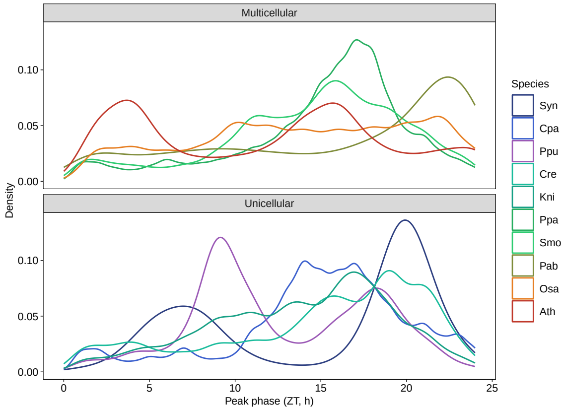
Peak-phase density: dawn/dusk enrichment across species
