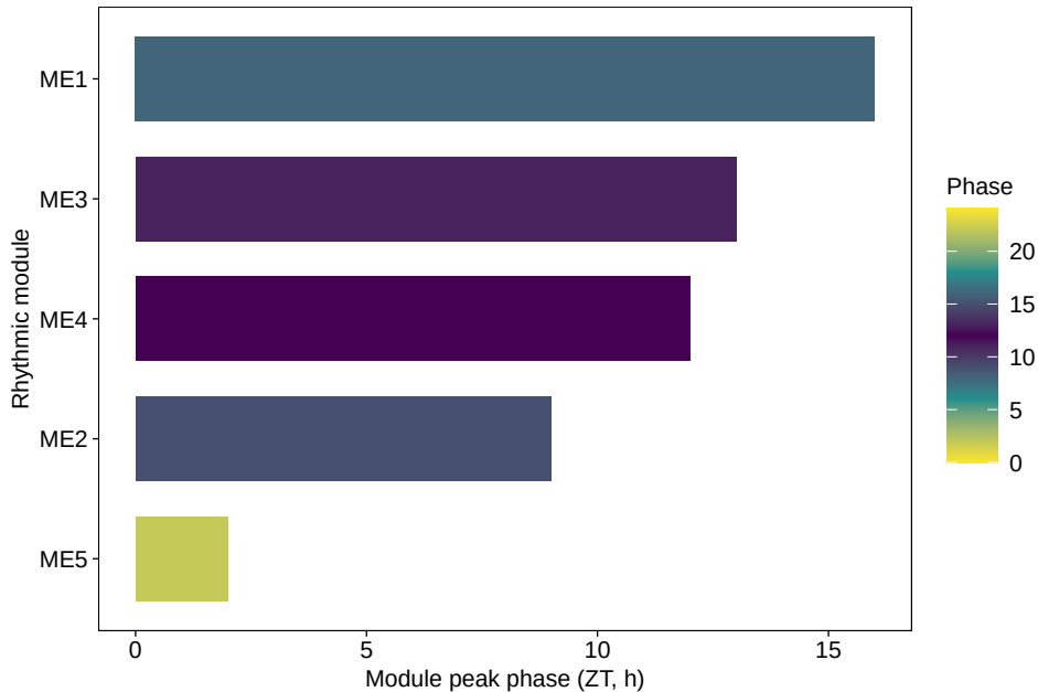
Klebsormidium nitens : co-expression modules by peak time
