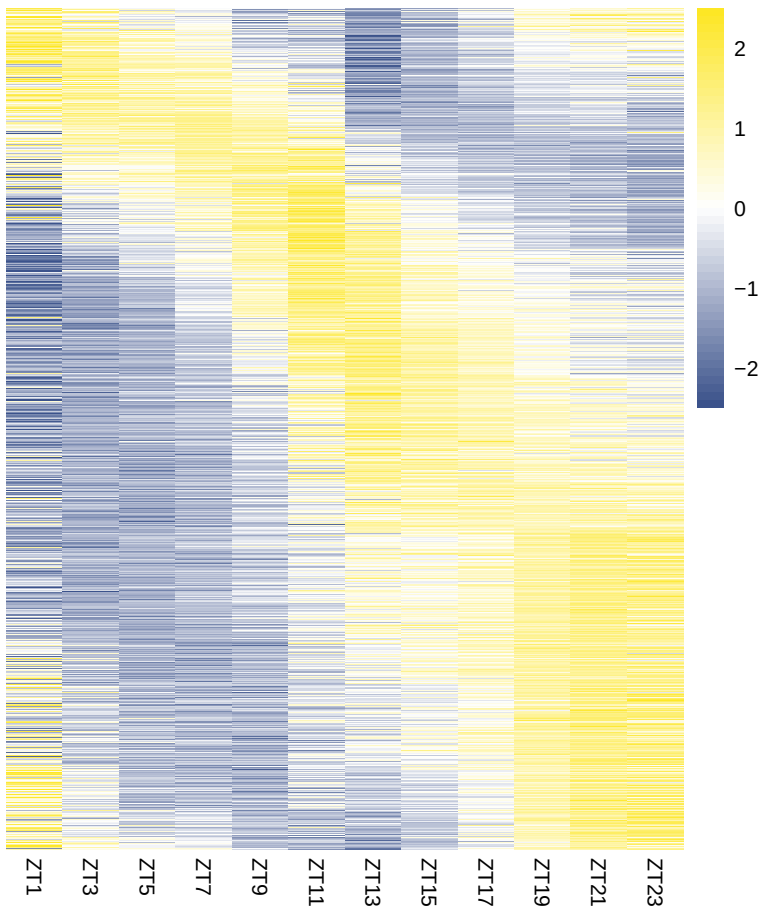
amydomonas reinhardtii rhythmic genes (sorted by phase)
