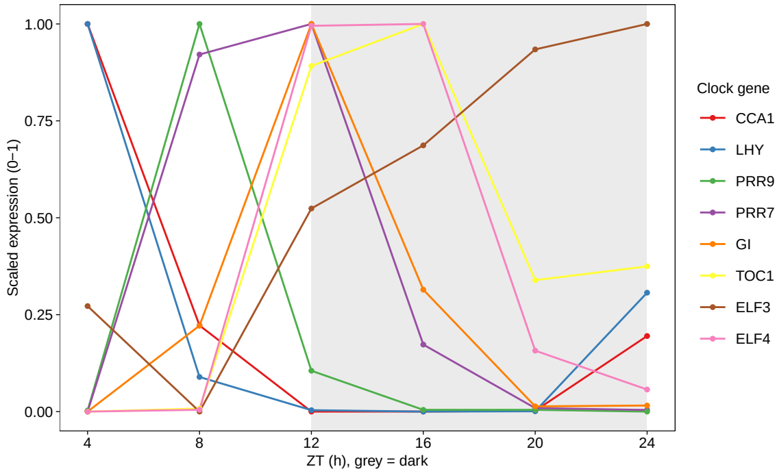
Arabidopsis core clock genes over the diurnal cycle
