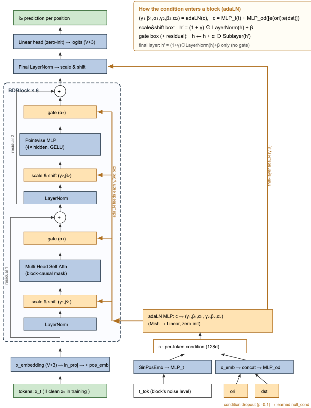
Figure 2. The denoiser is a standard DiT tower (Peebles & Xie style), read bottom-up. Each of the 6 blocks has two sublayers — self-attention, then a pointwise MLP — each wrapped as x \leftarrow x + \alpha \cdot \text{Sublayer}(x \cdot \text{LN}(x) + \beta) . The block's LayerNorms are affine-free ; all of \gamma ( scale ), \beta ( shift ), \alpha ( gate ) are produced by that block's zero-initialised adaLN MLP from the per-token condition c = \text{MLP}_t(t) + \text{MLP}_{od}([e(\text{ori}); e(\text{dst})]) . So the "6 modulations" map to precise insertion points: \gamma_1, \beta_1 rescale/shift the LayerNorm output fed into attention and \alpha_1 gates the attention output before the residual add; \gamma_2, \beta_2, \alpha_2 do the same for the MLP sublayer . The final LayerNorm before the head gets its own \gamma, \beta (no gate). Zero-init makes every block start as the identity. Because t is per token and each canvas block carries its own noise level, one forward pass handles blocks at different corruption stages — enabling the concatenated [x_t \parallel x_0] training pass (Fig. 1B) and semi-AR sampling with frozen ( t = 0 ) committed blocks. Differences from vanilla DiT: block-structured attention masks, a token head over V+3 states instead of patch reconstruction, and the OD embedding added into c alongside the timestep.
