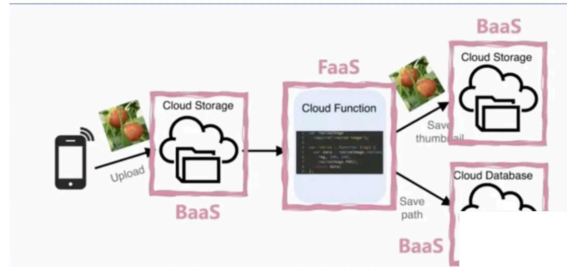
Serverless
