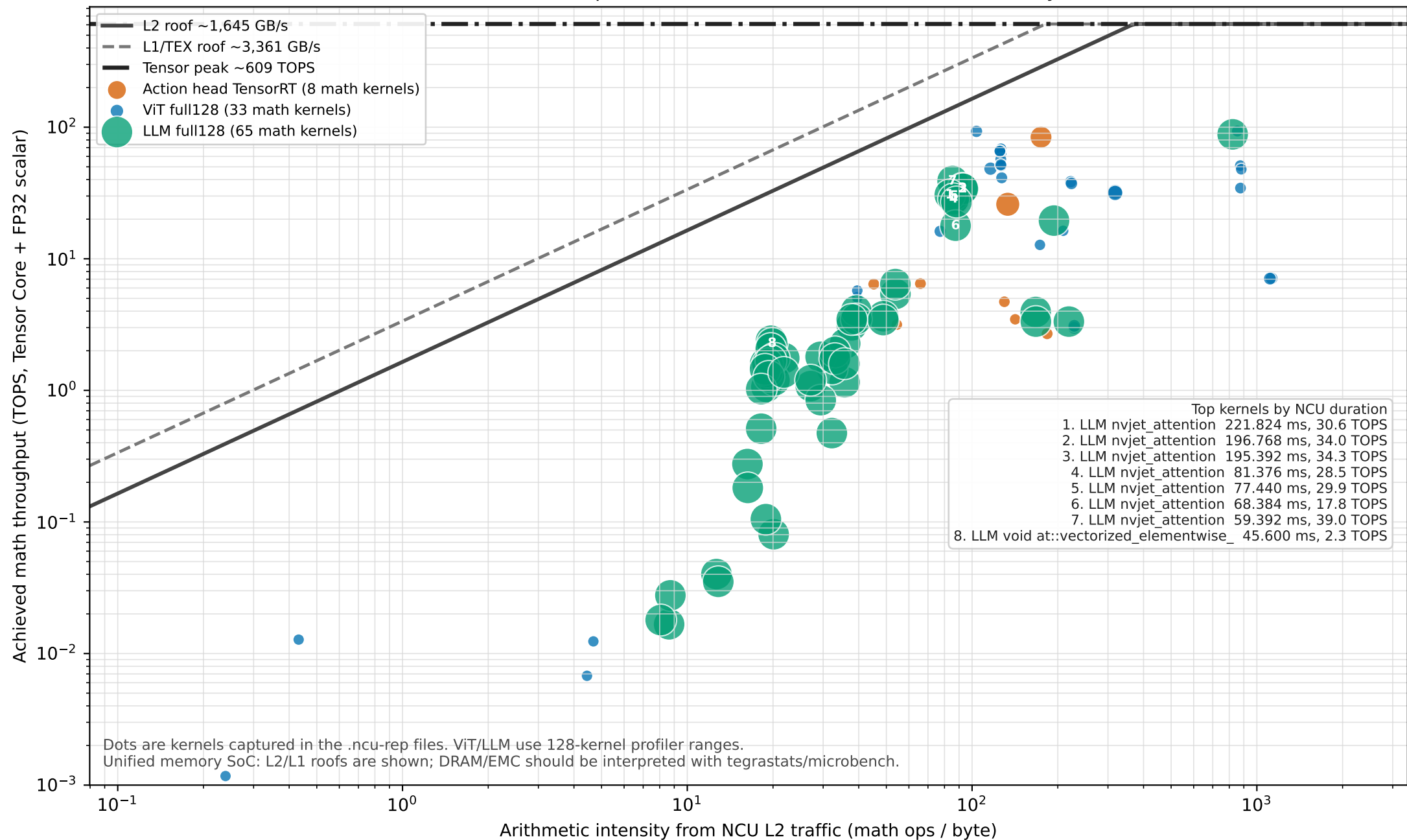
GR00T N1.6 NCU-Rep Roofline, Governor Clocks, Unified Memory Thor
