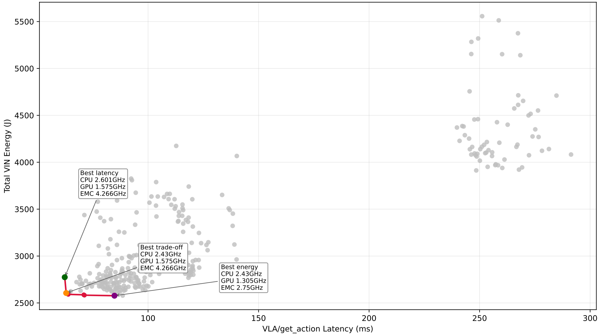
Pareto Front: Latency vs Total VIN Energy (All-default removed)
