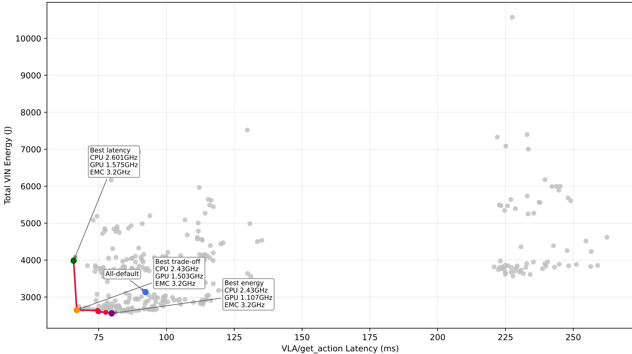
Pareto Front: Latency vs Total VIN Energy (All-default shown)
