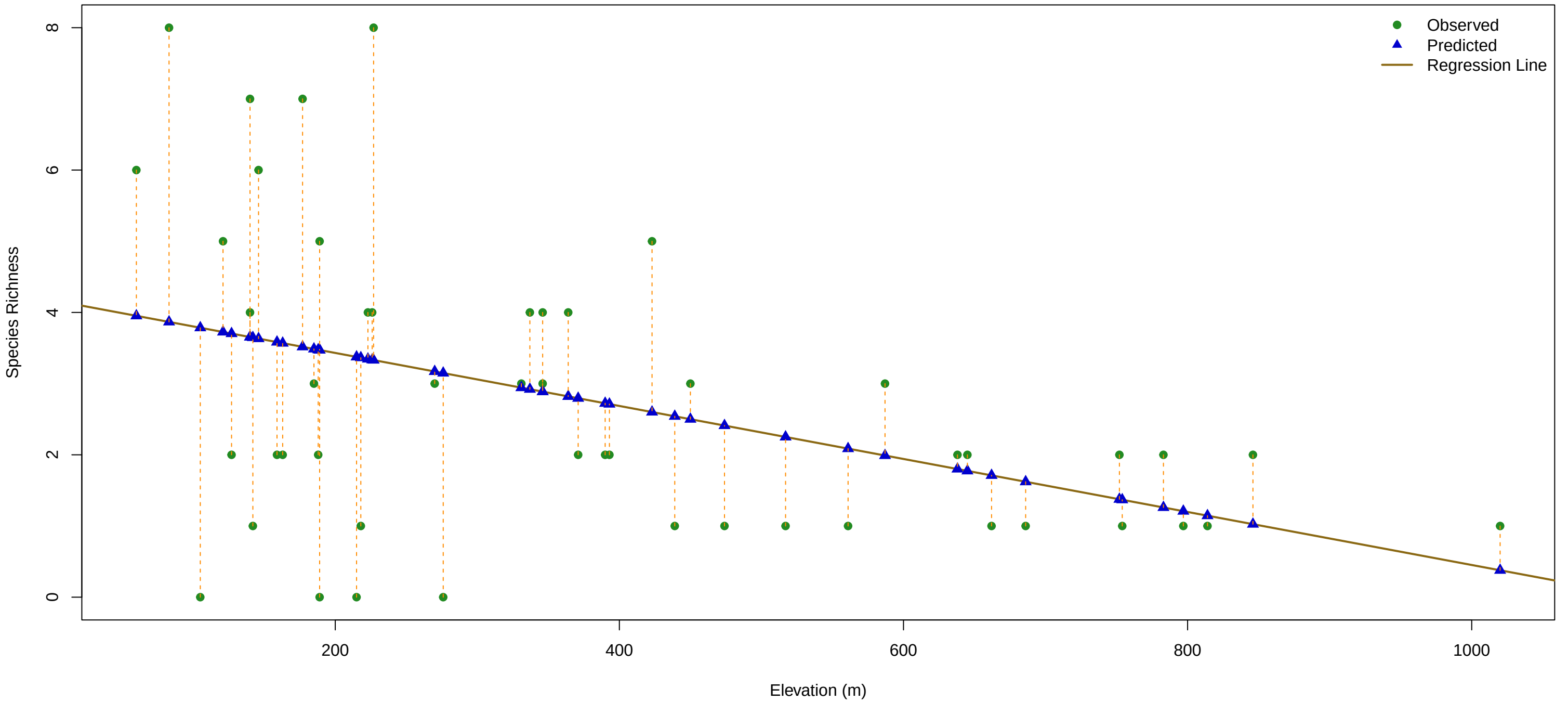
Simple Linear Regression Model
