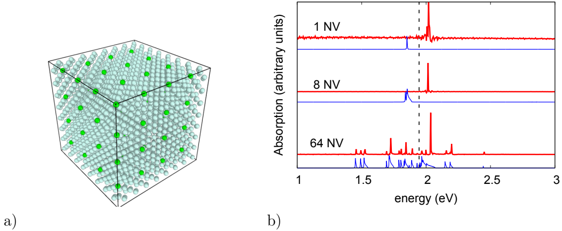
Figure 5: Concentration dependence of the optical response in parallel-aligned NV − arrays. Spin-collinear RT-TDDFT spectra are shown in red and independent-particle approximation (IPA) spectra, evaluated with the LOPTICS implementation in RMG, are shown in blue. From top to bottom, the systems contain 1, 8, and 64 NV − centers in the same 4096-site diamond host, corresponding to the NV- x8 , NV- x4 , and NV- x2 defect concentrations, respectively. All calculations use the same atomic structures, real-space grid, \Gamma -point representation, transverse polarization, and spectral broadening. The RT-TDDFT calculations additionally use the same retained occupied fraction and number of virtual states per diamond site and were propagated for 42000 steps with \Delta t = 1.0 a.u., corresponding to approximately 1.02 ps. The dashed vertical line marks the experimental zero-phonon-line energy, E_{\text{ZPL}} = 1.945 eV. The strongly fragmented spectrum of the 64-NV array reflects substantial coupling among closely spaced defects. At the 8-NV concentration, the IPA retains nearby independent-particle transition structure, whereas the RT-TDDFT response is dominated by a single resonance resembling that of the dilute single-NV system. The spectra are vertically offset, and the IPA curves are independently scaled, for clarity.
