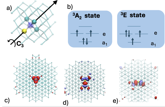
Figure 2: Electronic structure of the negatively charged NV^- center in diamond. (a) Local atomic structure of the defect, consisting of a substitutional nitrogen atom adjacent to a carbon vacancy. The arrow indicates the [111] direction, which defines the C_3 axis of the approximately C_{3v} defect. (b) Schematic occupation of the defect levels in the triplet ground-state configuration, a_1^2 e_x^1 e_y^1 , and in the defect-associated optically excited triplet configuration. The experimental 1.945 eV ZPL is used in this work only as a reference energy for the defect-region response. (c–e) Representative real-space isosurfaces of Kohn–Sham defect orbitals localized in the diamond band gap: the occupied a_1 -like orbital and the two components of the nearly degenerate e manifold.
