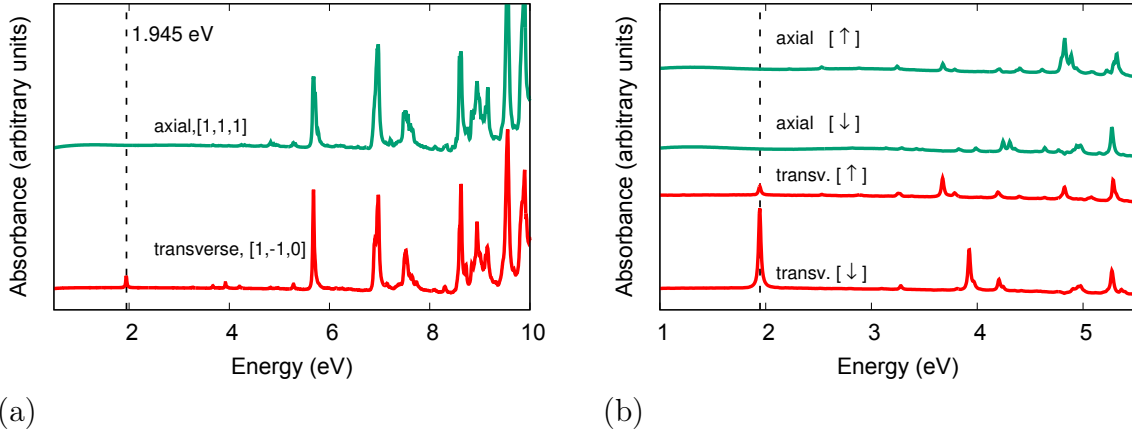
Figure 3: Polarization and spin selectivity of the NV - defect optical response from spin-collinear RT-TDDFT for the 512-site NV- x4 supercell. The spectra are optical spectra in arbitrary units and are vertically shifted for clarity. (a) Spin-summed response for a perturbation parallel to the NV axis, [111] , and for a transverse perturbation along [1\bar{1}0] . The dashed vertical line marks the experimental NV - ZPL energy, E_{\text{ZPL}} = 1.945 eV, as a reference. The defect-associated feature near this energy is strongly enhanced for transverse polarization and suppressed for axial polarization. (b) Expanded spin-resolved view of the sub-gap response. In the global spin convention used here, the transverse response near the ZPL reference is dominated by the spin-down channel, consistent with a local minority-spin a_1 \rightarrow e excitation.
