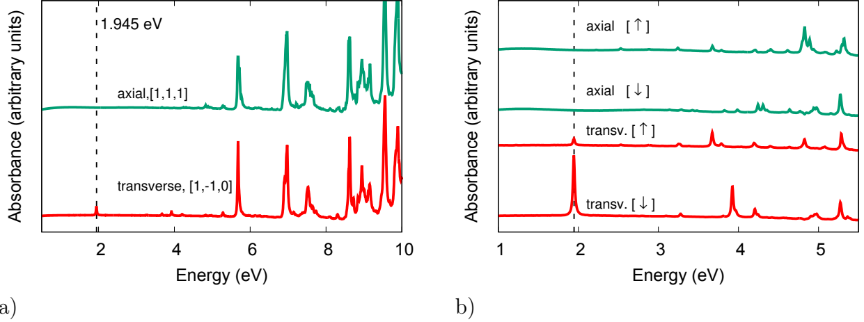
Figure 3: Polarization and spin selectivity of the NV - defect optical response from spin-collinear RT-TDDFT for the 512-site NV- x 4 supercell. (a) Spin-summed spectra for axial and transverse light polarizations. The axial spectrum corresponds to a kick polarized parallel to the NV axis, \mathbf{E} \parallel [111] , while the transverse spectrum corresponds to \mathbf{E} \parallel [1\bar{1}0] , perpendicular to the NV axis. The dashed vertical line marks the experimental NV - zero-phonon-line energy, E_{\text{ZPL}} = 1.945 eV. The defect-associated peak near this energy is strongly enhanced for transverse polarization and suppressed for axial polarization, consistent with the C_{3v} selection rule for the {}^3A_2 \rightarrow {}^3E transition. (b) Expanded view of the sub-gap optical response below approximately 5.5 eV, corresponding to the transparency window of pristine diamond. In this energy range, optical features arise from the NV - defect states rather than from intrinsic band-to-band absorption of the diamond host. The spin-resolved spectra show that the transverse response near the ZPL energy is dominated by the spin-down, minority-spin channel, consistent with the dominant a_1 \rightarrow e defect excitation shown schematically in Fig. 2. The spectra are vertically shifted for clarity.
