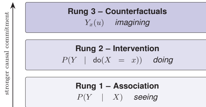
Figure 3.1: Pearl’s ladder of causation: each rung answers a strictly stronger class of questions [PM18].
