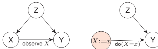
Figure 3.2: Observing X leaves the confounding path through Z intact; intervening on X severs its incoming edges.
