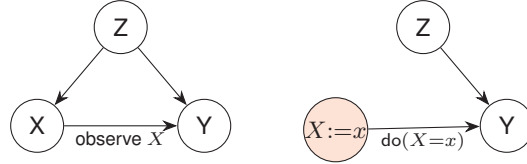
Figure 3.2: Observing X leaves the confounding path through Z intact; intervening on X severs its incoming edges (Definition A.3.25).
