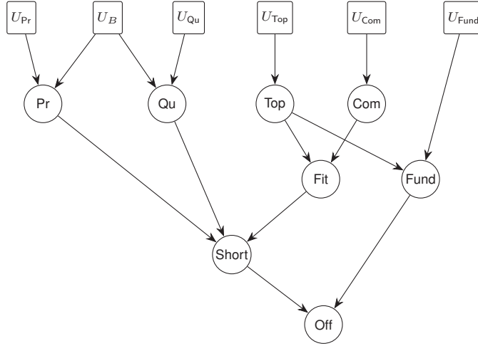
Figure A.3: The explicit all-directed graph of Mira’s latent causal skeleton. Rectangles are exogenous roots and circles are endogenous nodes. The shared root U_B is incident to both Pr and Qu ; no bidirected edge is primitive in this representation.
