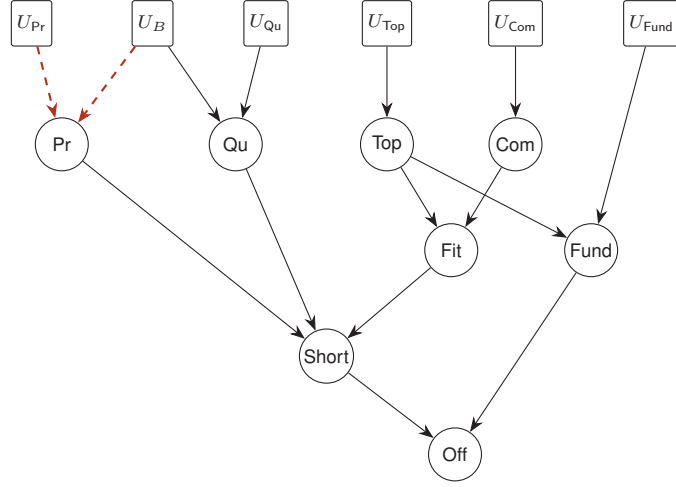
Figure A.4: Incoming arrows into \text{Pr} under \mathcal{G}_{\text{Mira}, \overline{\text{Pr}}} . Dashed coloured arrows U_{\text{Pr}} \rightarrow \text{Pr} and U_B \rightarrow \text{Pr} are marked for deletion; U_B \rightarrow \text{Qu} and \text{Pr} \rightarrow \text{Short} are retained.
