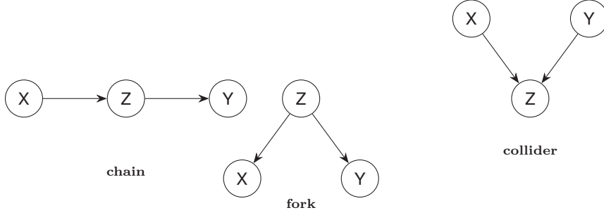
Figure A.2: The three local directed configurations of Definition A.4.4. The middle node is a non-collider in a chain or fork and a collider in the final configuration.
