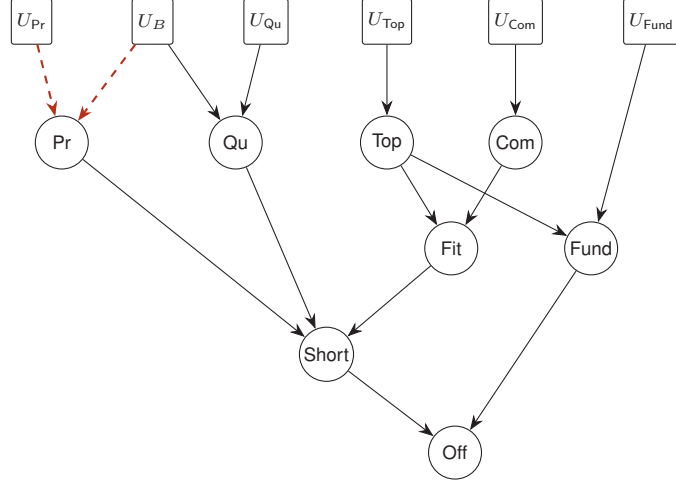
Figure A.4: Incoming arrows into Pr under \mathcal{G}_{Mira, \overline{Pr}} . Dashed coloured arrows U_{Pr} \rightarrow Pr and U_B \rightarrow Pr are marked for deletion; U_B \rightarrow Qu and Pr \rightarrow Short are retained.
