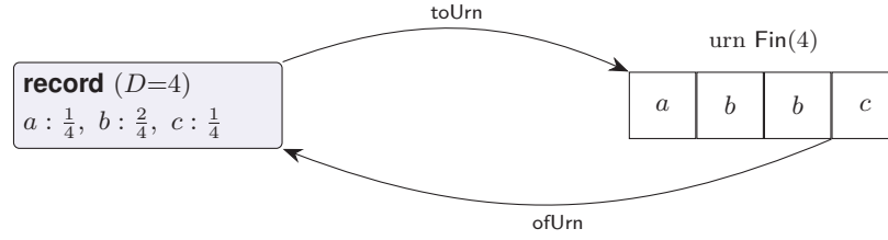
Figure B.1: Record and urn presentations of a finite rational distribution agree on every decidable event (Proposition B.6.11); the maps toUrn/ofUrn are the computable witnesses checked in Lean.
