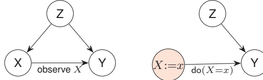
Figure 3.2: Observing X leaves the confounding path through Z intact; intervening on X severs its incoming edges (Definition A.4.16).
