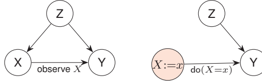
Figure 3.2: Observing X leaves the confounding path through Z intact; intervening on X severs its incoming edges (Definition A.4.17).
