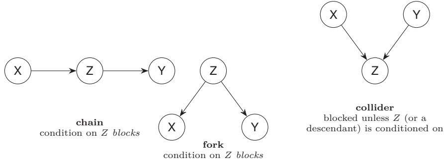
Figure A.1: The three path configurations behind d-separation (Definitions A.4.9 and A.4.11): chains and forks are non-colliders (conditioning on the middle node blocks the path); a collider blocks the path by default and is opened by conditioning on it or any of its descendants.
