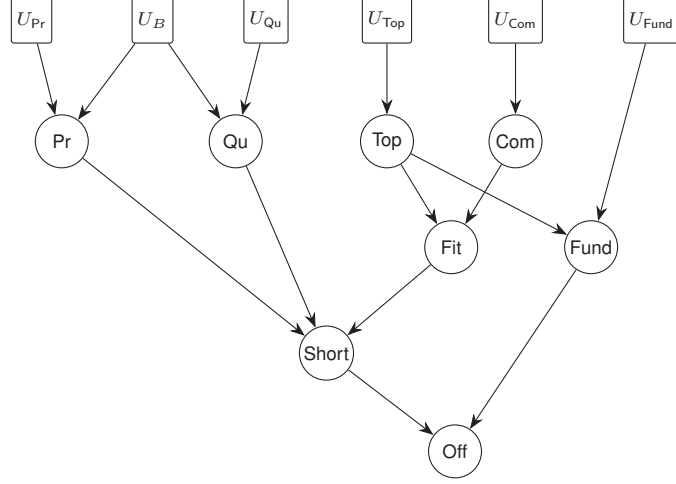
Figure A.3: The explicit all-directed skeleton of Mira's finite latent causal signature. Rectangles are exogenous roots and circles are endogenous nodes. The shared root U_B is incident to both \text{Pr} and \text{Qu} ; no bidirected edge is primitive in this representation.
