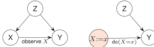
Figure 3.2: Observing X leaves the confounding path through Z intact; intervening on X severs its incoming edges (Definition A.4.23).
